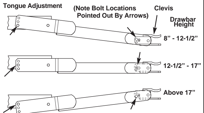
Figure 2-2 Tongue/Clevis Adjustment
