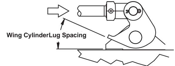
Figure 3-2 Make Sure Cylinders Are Fully Extended To Allow Decks To Float
