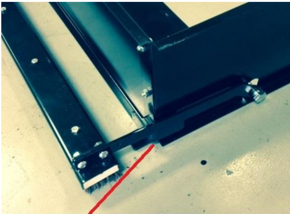
Lift tab goes here and is held on with 5/16 flange nut provided, one must tighten via the bolt and not the flange nut
